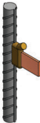
BRE60 (Vertical Tape End Tap to Rebar)
